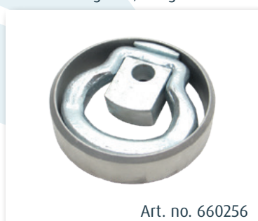
Recessed lashing ring Alloy recessed, steel ring. 4000 kg. \varnothing 92x23 mm. Nut (660255) not incl. Weight: 0,44 kg
